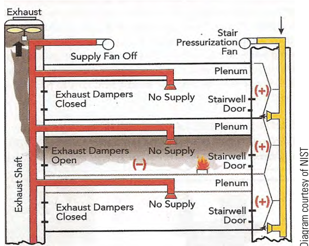
Figure 12.11. A diagram of an exhaust system (left) and a stair pressurization system (right).
