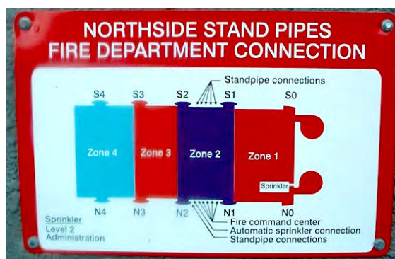
Figure 10.4. A sign indicating the areas covered by separate manual dry standpipe systems. The colors and zone numbers correspond to zones with separate FDCs.
