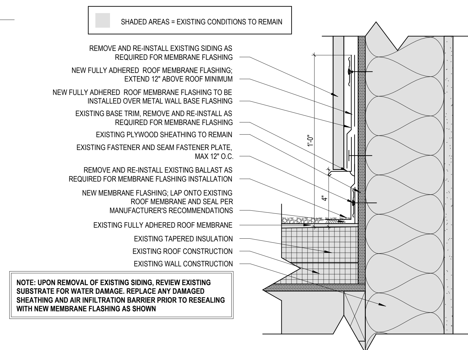
6 Roof to Wall Detail Scale: 3" = 1'-0"
