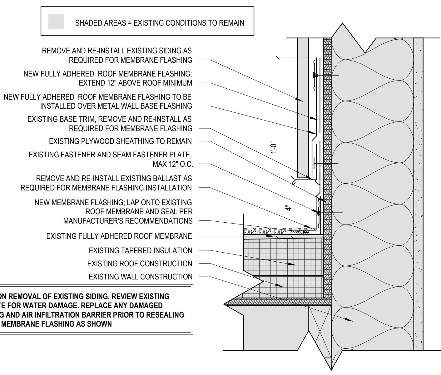
6 Roof to Wall Detail Scale: 3" = 1'-0"
