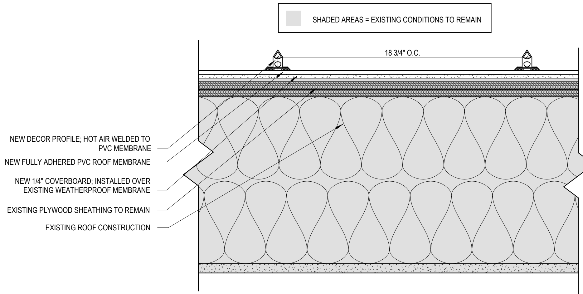
2 Typical Roof Section Scale: 3" = 1'-0"
