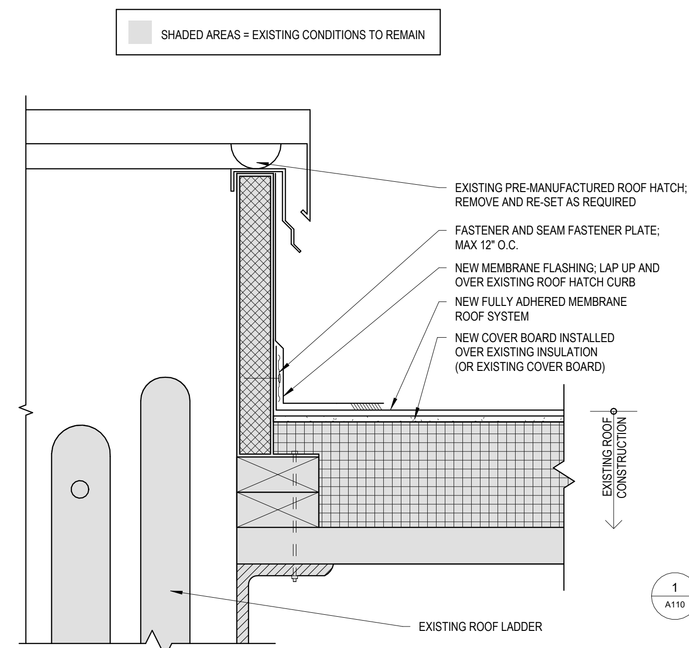
4 Roof Hatch Detail Scale: 3" = 1'-0"
