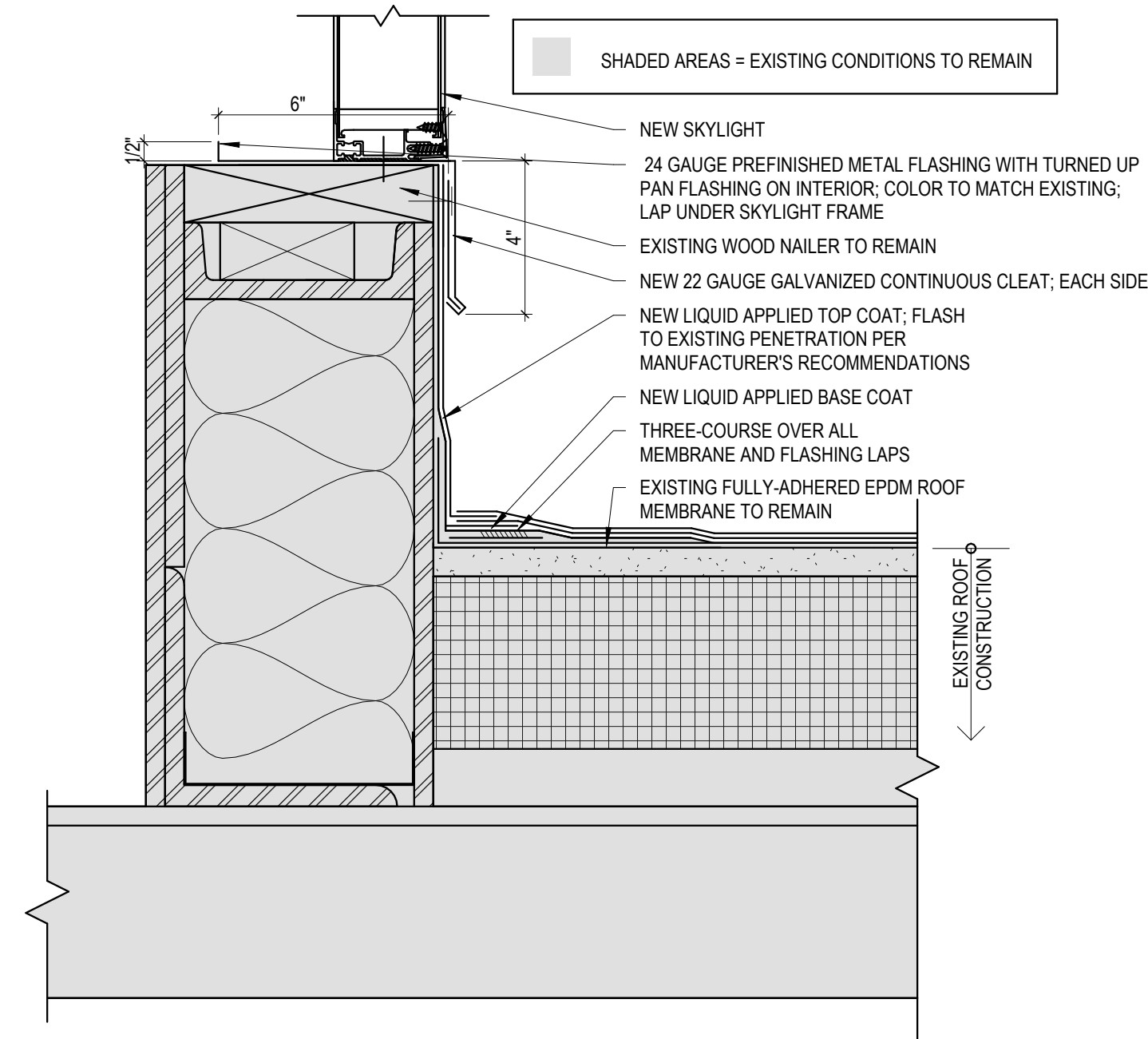
6 Skylight Roof Curb Detail - Alt. Bid #1 Scale: 3" = 1'-0"
