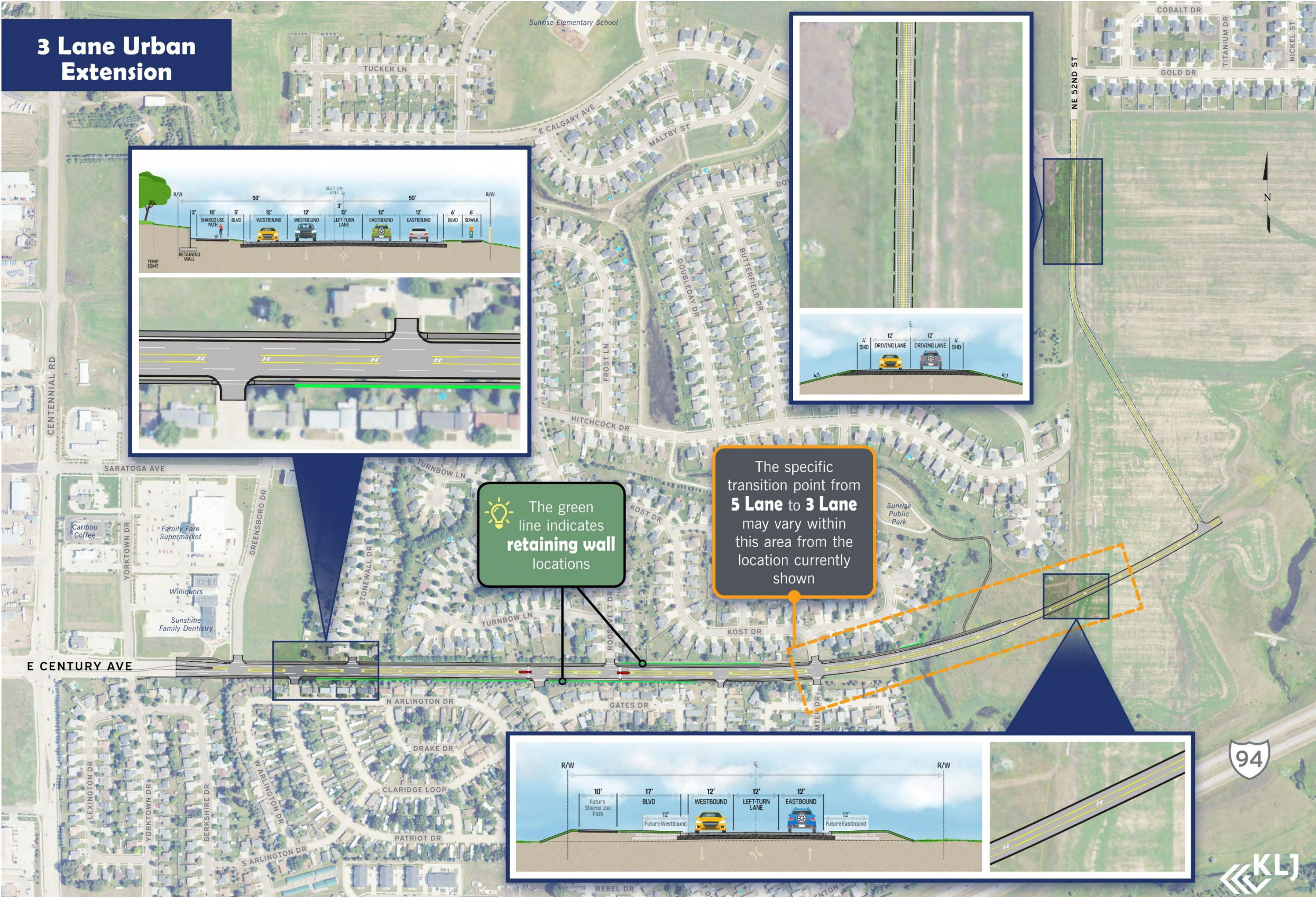
Exhibit 8, Alternative D: 5-Lane with 3 Lane Urban Extension
