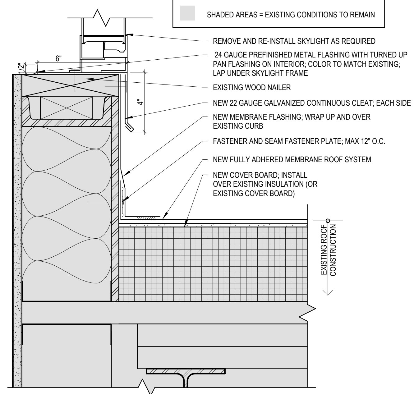
2 Roof Curb at Skylight Detail Scale: 3" = 1'-0"
