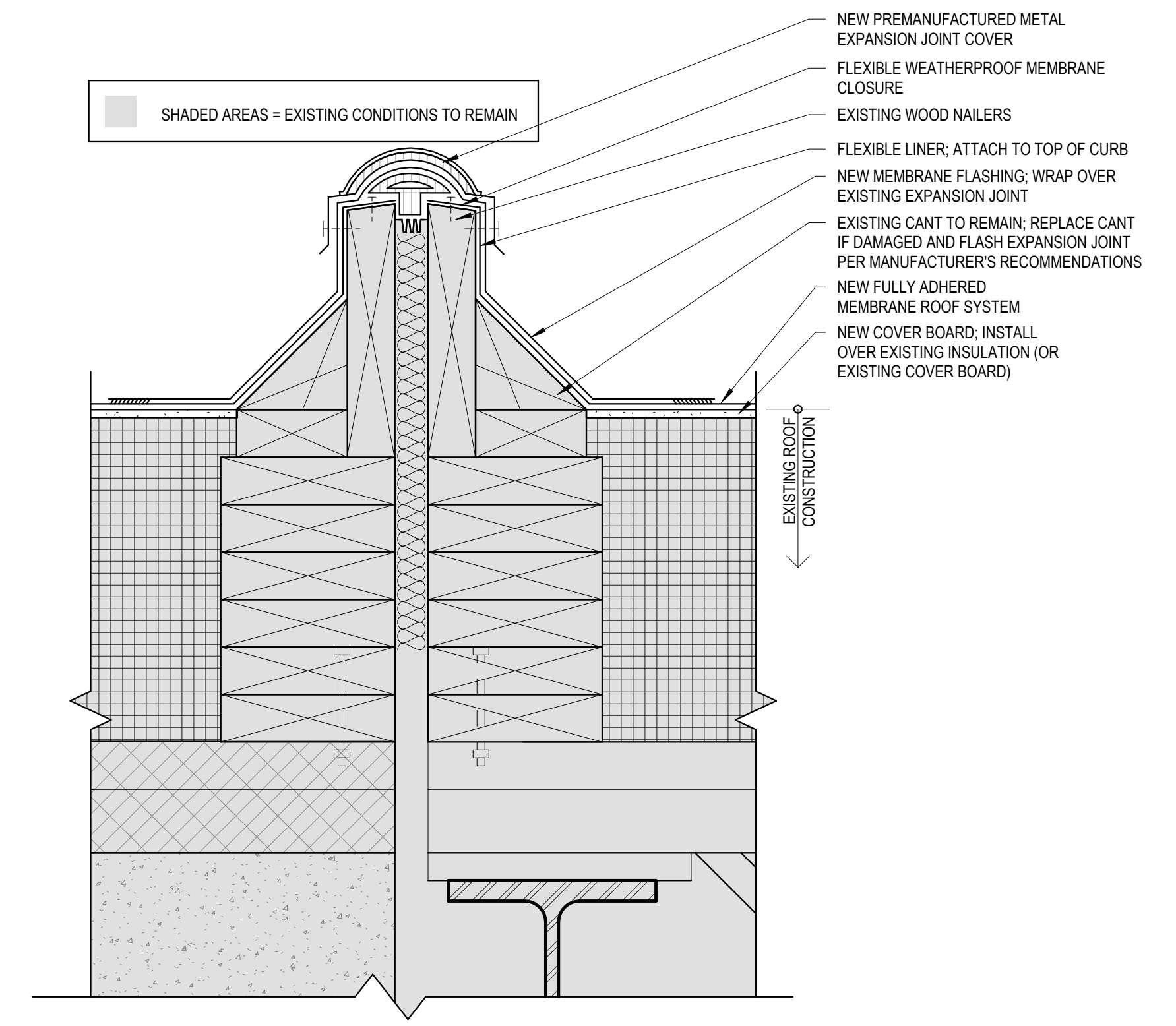
4 Roof Expansion Joint Detail Scale: 3" = 1'-0"
