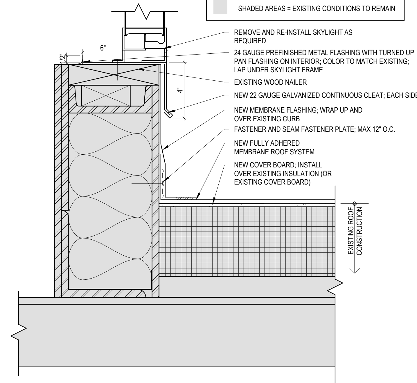
3 Roof Curb at Skylight Detail Scale: 3" = 1'-0"
