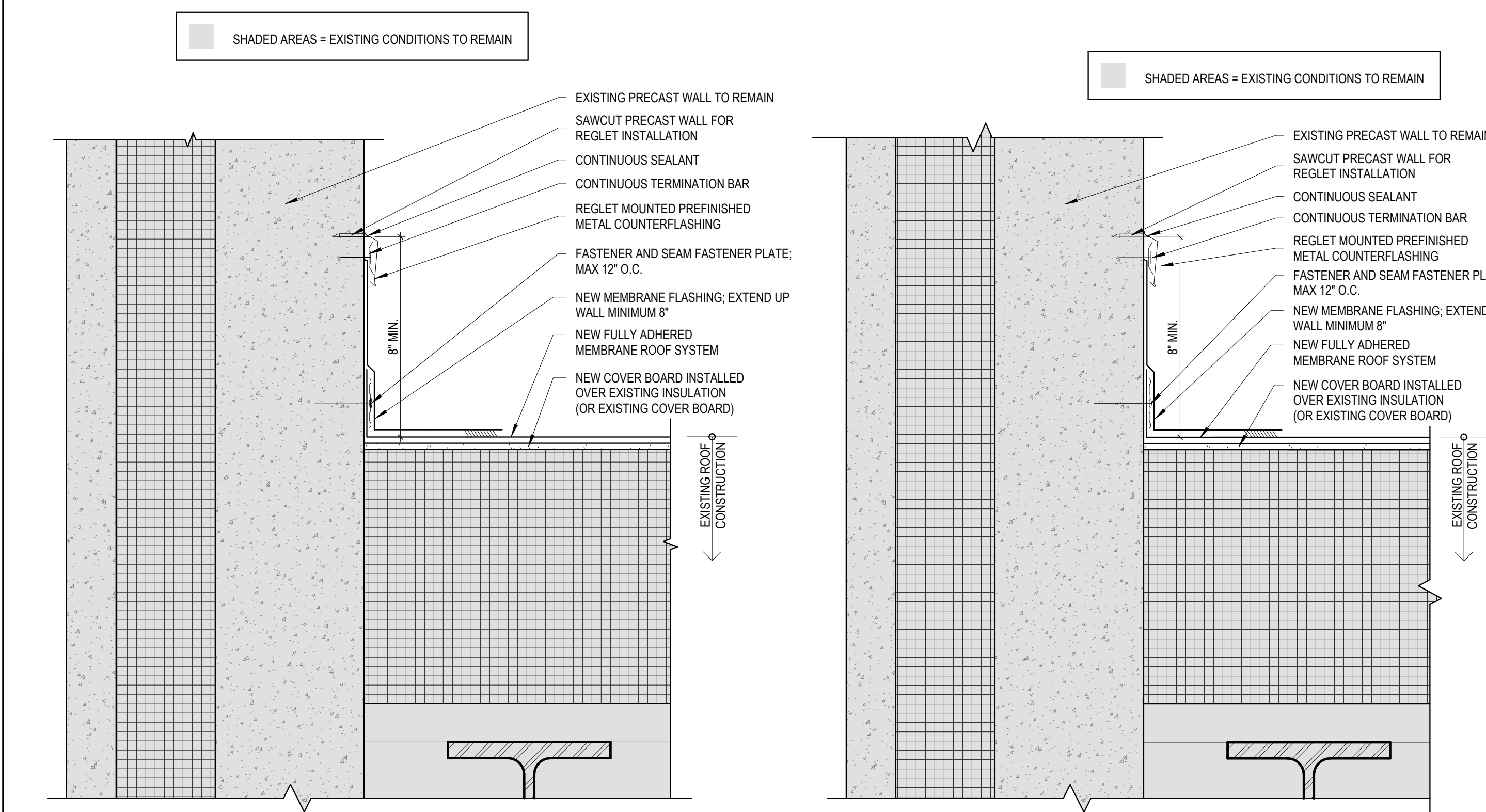
2 Roof Counterflashing Detail Scale: 3" = 1'-0"
