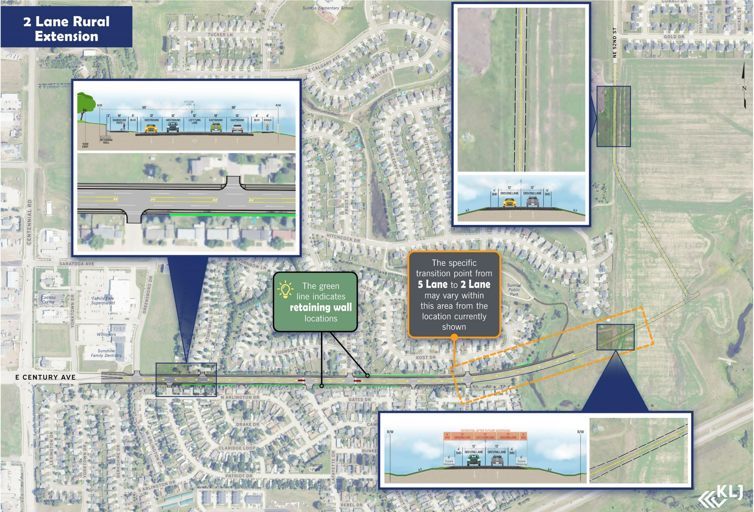
Exhibit 7, Alternative C: 5-Lane with 2 Lane Rural Extension
