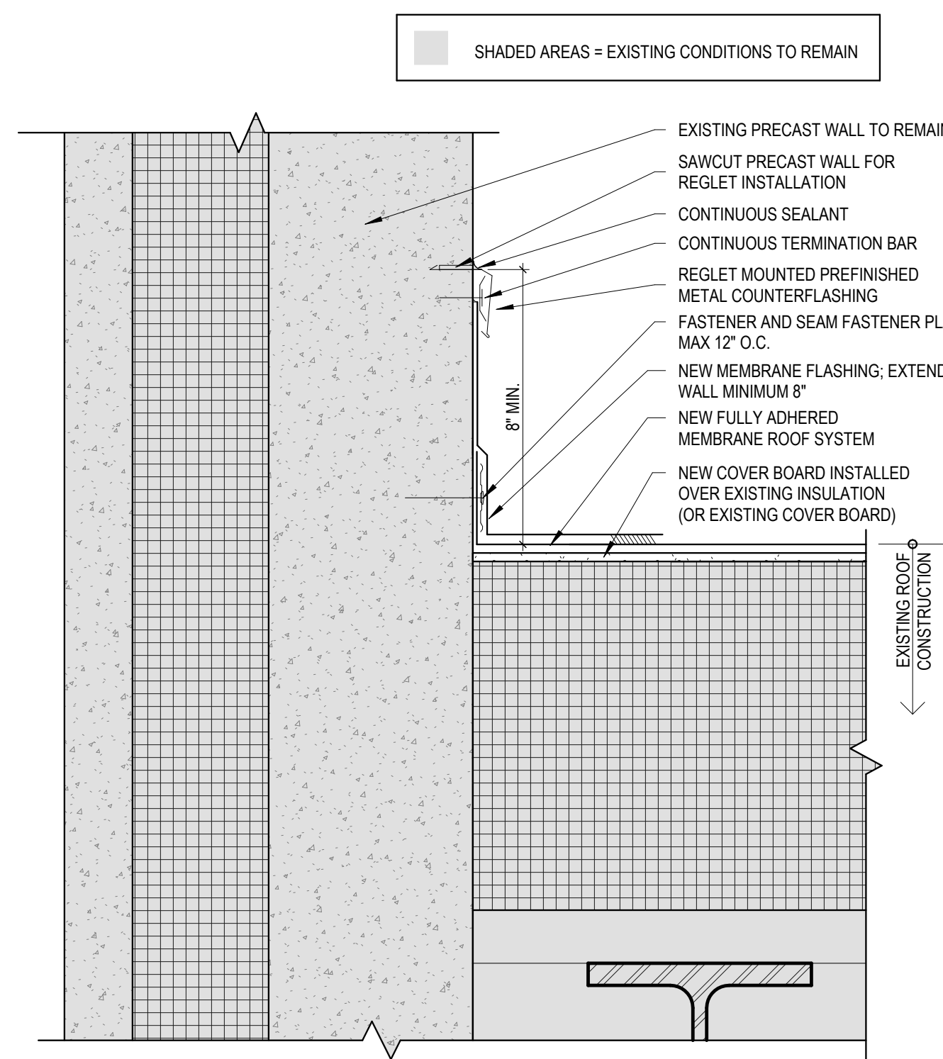
3 Roof Counterflashing Detail Scale: 3" = 1'-0"
