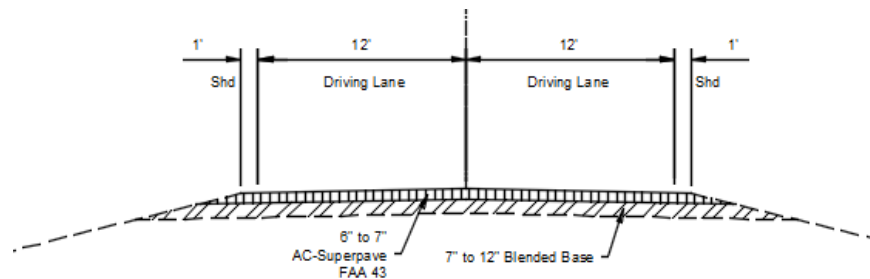
Existing Typical Section E Century Ave
