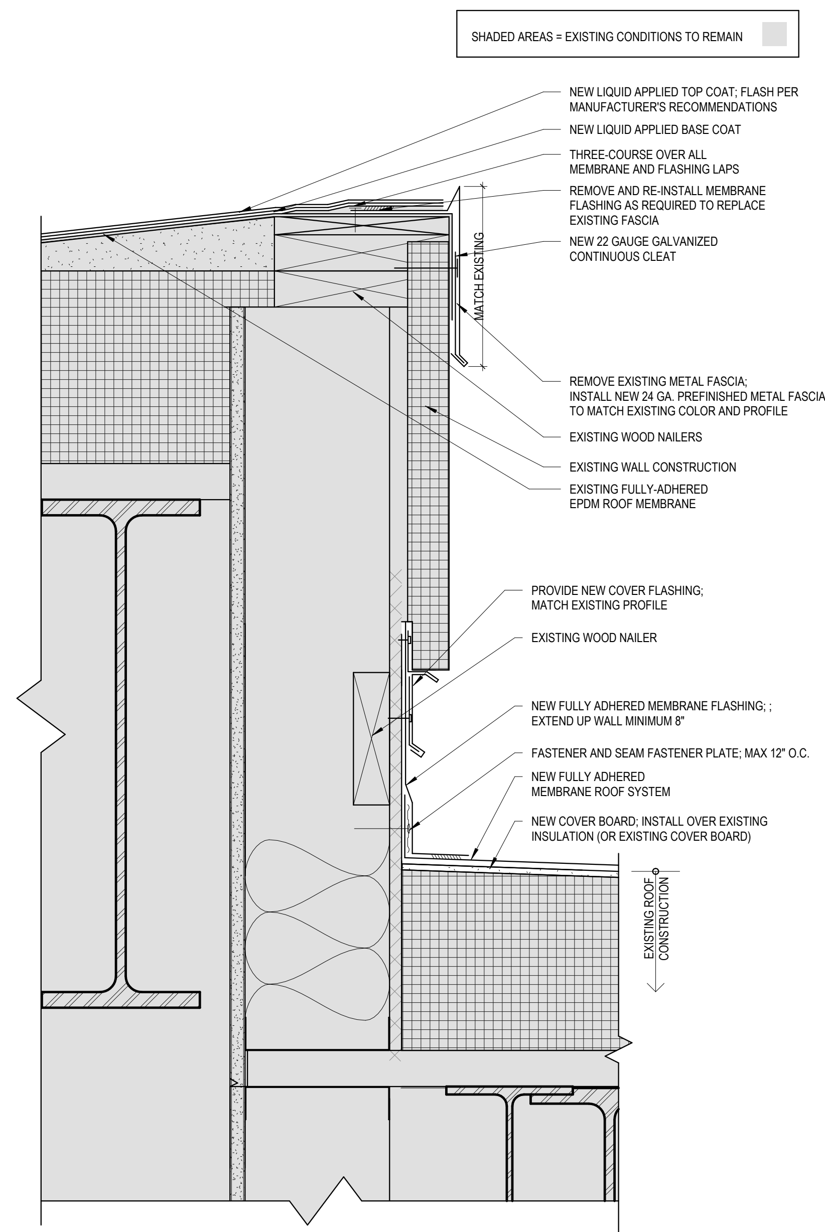
5 Roof Expansion Joint Detail Scale: 3" = 1'-0"
