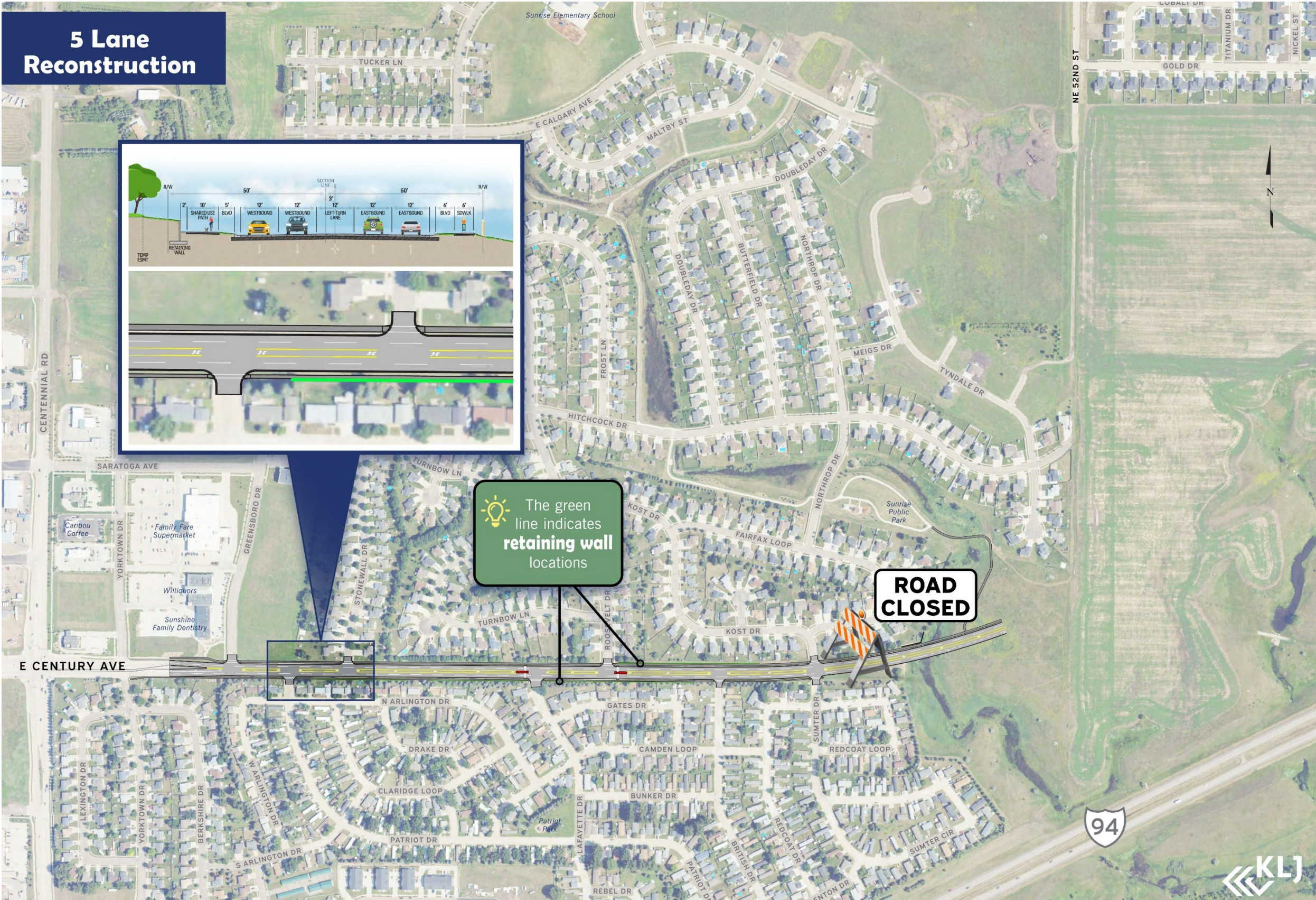
Exhibit 6, Alternative B: 5-Lane Reconstruction
