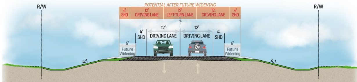
Exhibit 4, 52 nd St NE extension to East Century Ave & Two-Lane Rural Section from east of Sunrise Tributary to 52nd St NE extension
