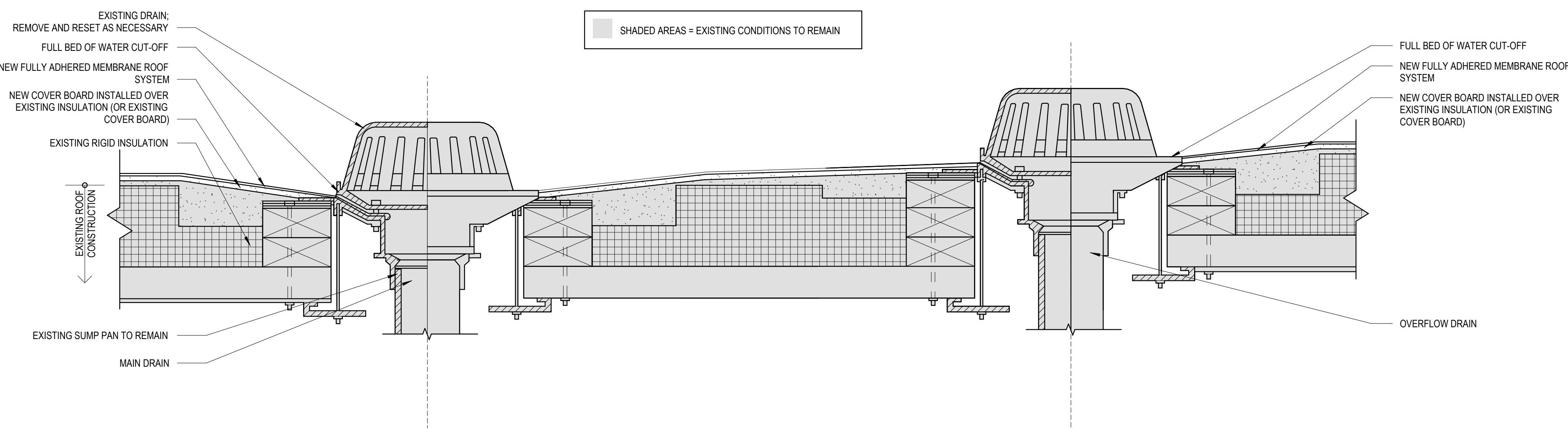
2 Typical Roof Drain and Overflow Drain Detail Scale: 3" = 1'-0"
