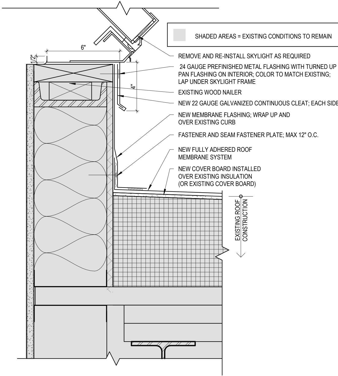
1 Roof Curb at Skylight Detail Scale: 3" = 1'-0"
