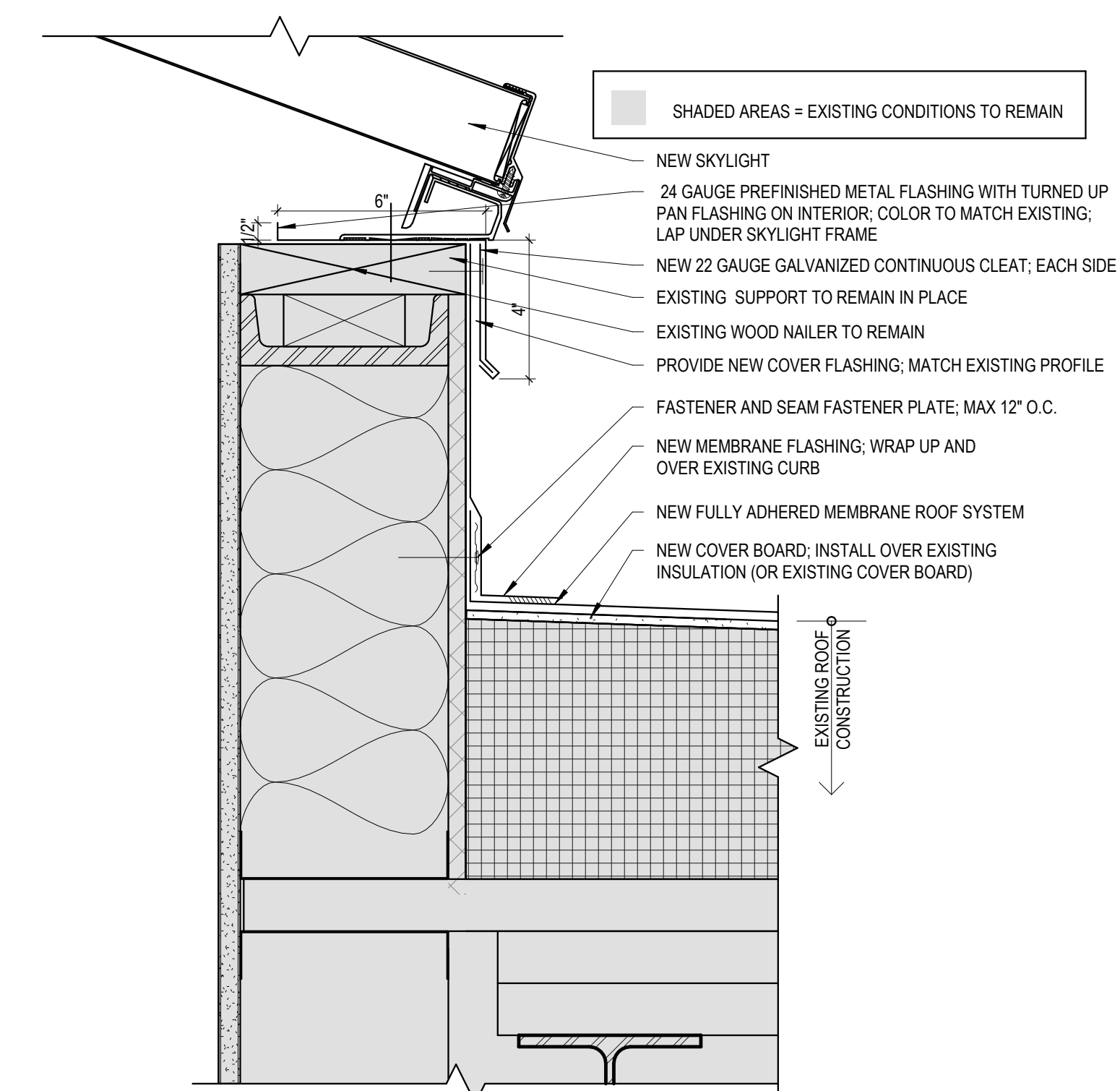
8 Skylight Roof Curb Detail - Alt. Bid #1 Scale: 3" = 1'-0"
