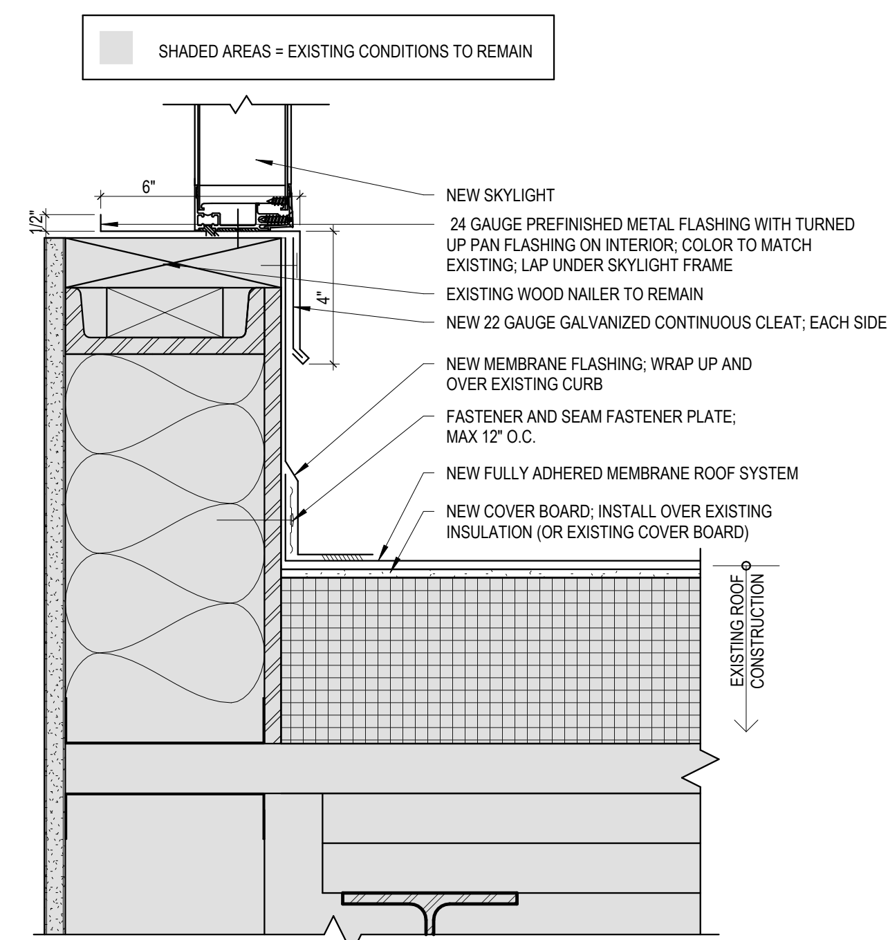
7 Skylight Roof Curb Detail - Alt. Bid #1 Scale: 3" = 1'-0"
