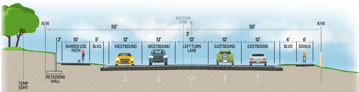
Exhibit 3, Five-Lane Typical Section from Greensboro Dr to East of Sunrise Tributary
