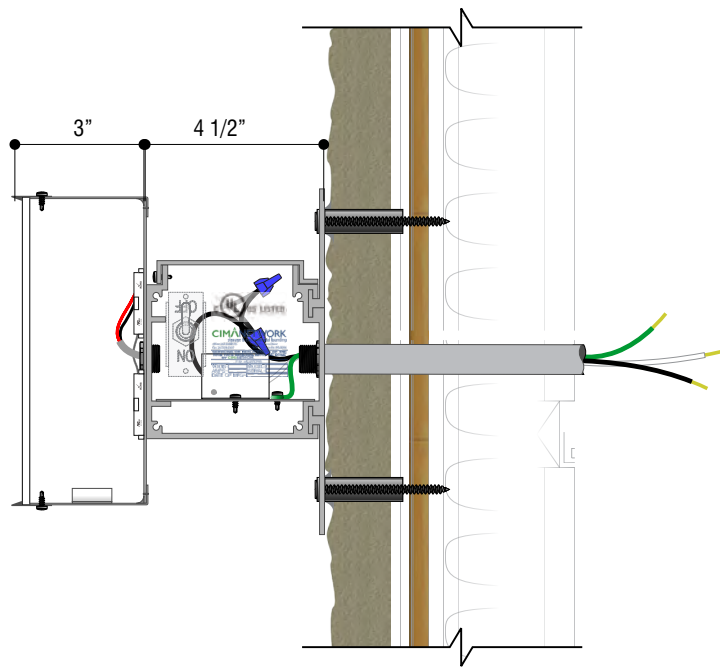
1.3 face-lit logo vertical section detail scale: 3" = 1'-0"
