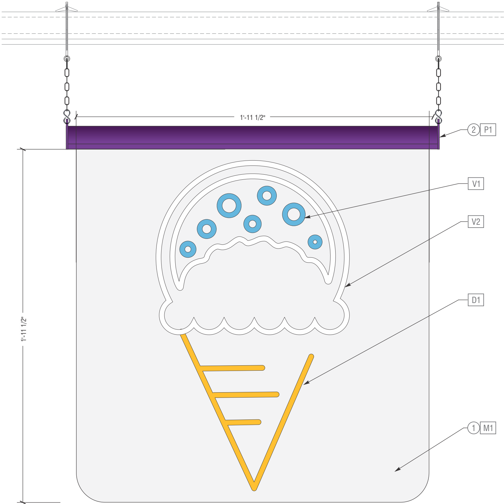
6.1 illuminated edge-lit hanging window sign
