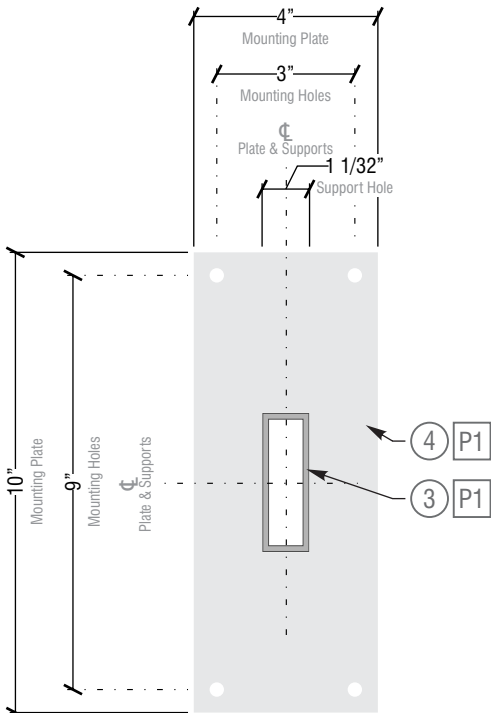
7.6 face-lit blade sign mounting plate detail scale: 3" = 1'-0"
