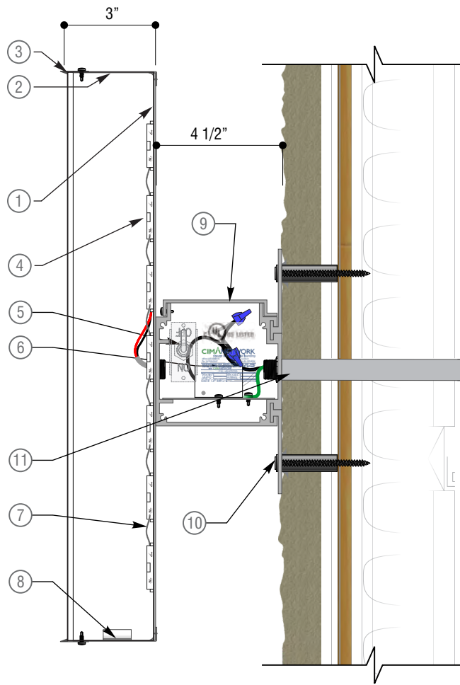
1.2 face-lit logo vertical section detail scale: 3" = 1'-0"
