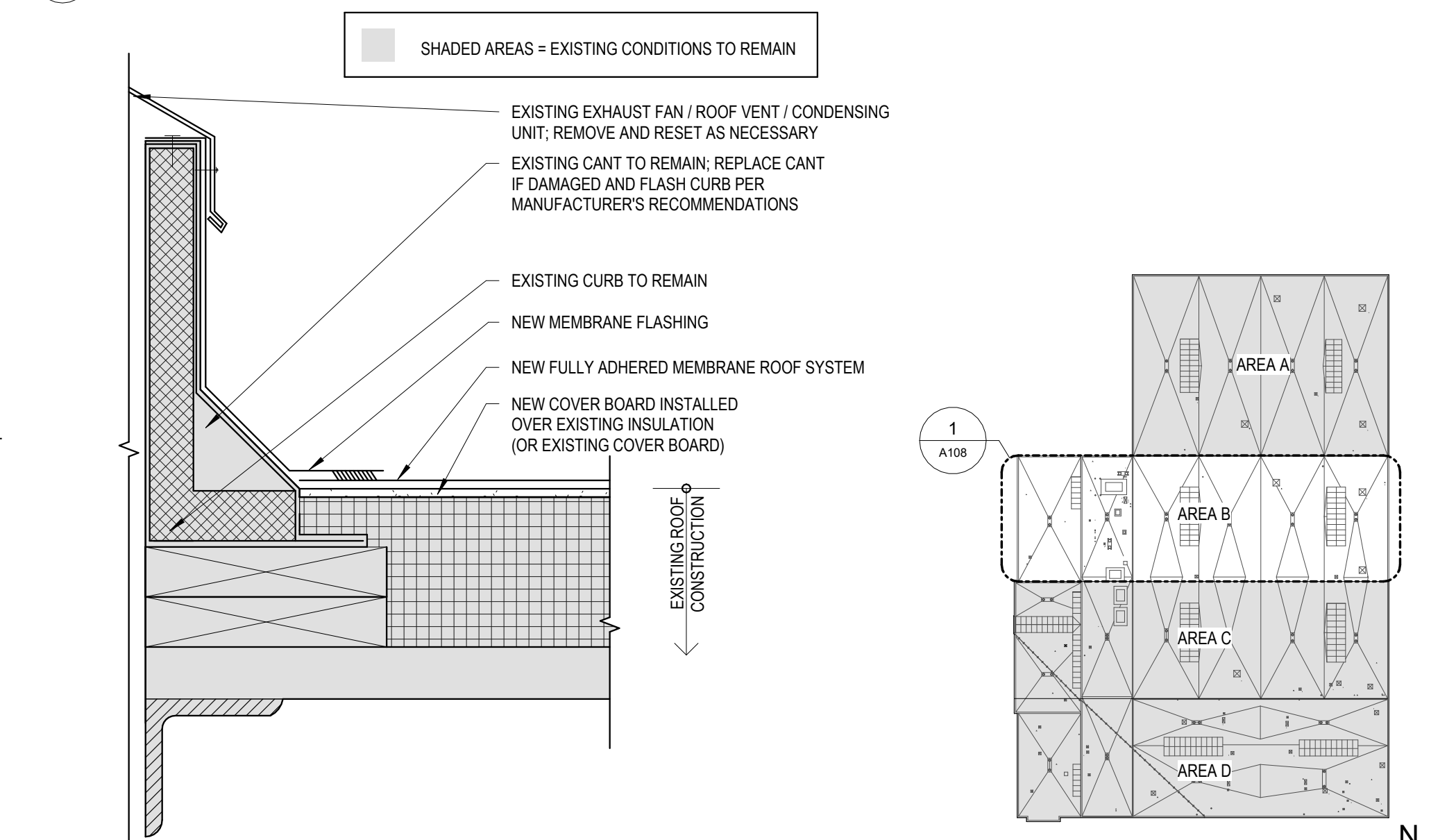
7 Typical Roof Curb Detail Scale: 3/4" = 1'-0"
