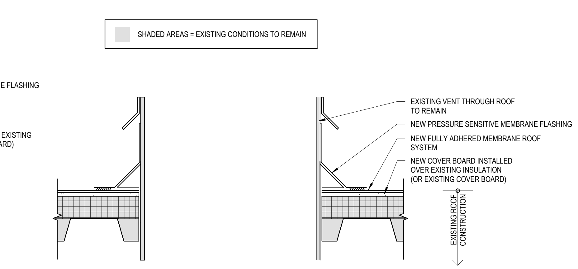
4 Typical Roof Vent Detail Scale: 3/4" = 1'-0"
