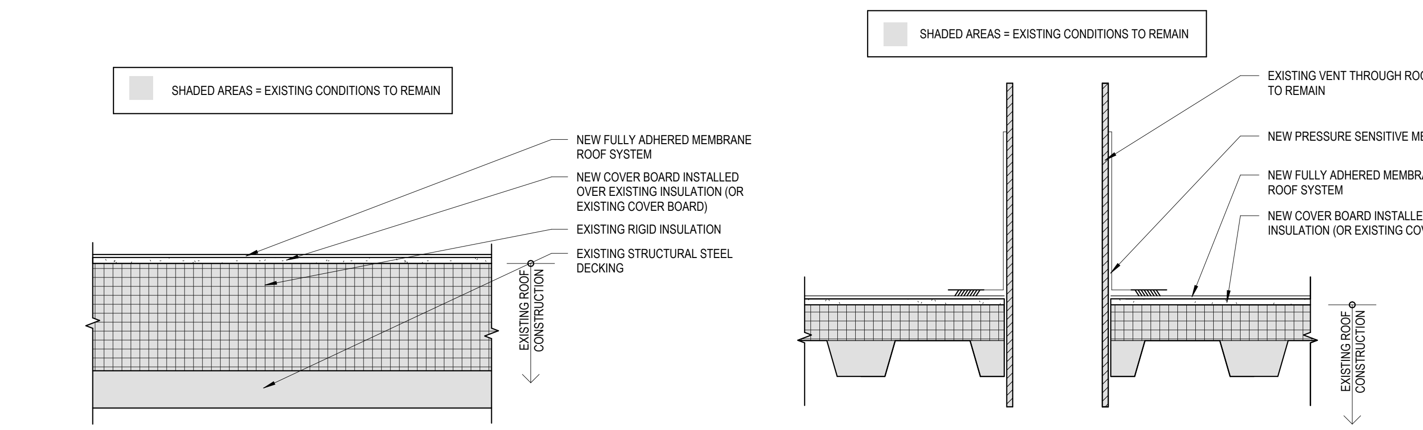
2 Typical Roof Section Scale: 3/4" = 1'-0"
