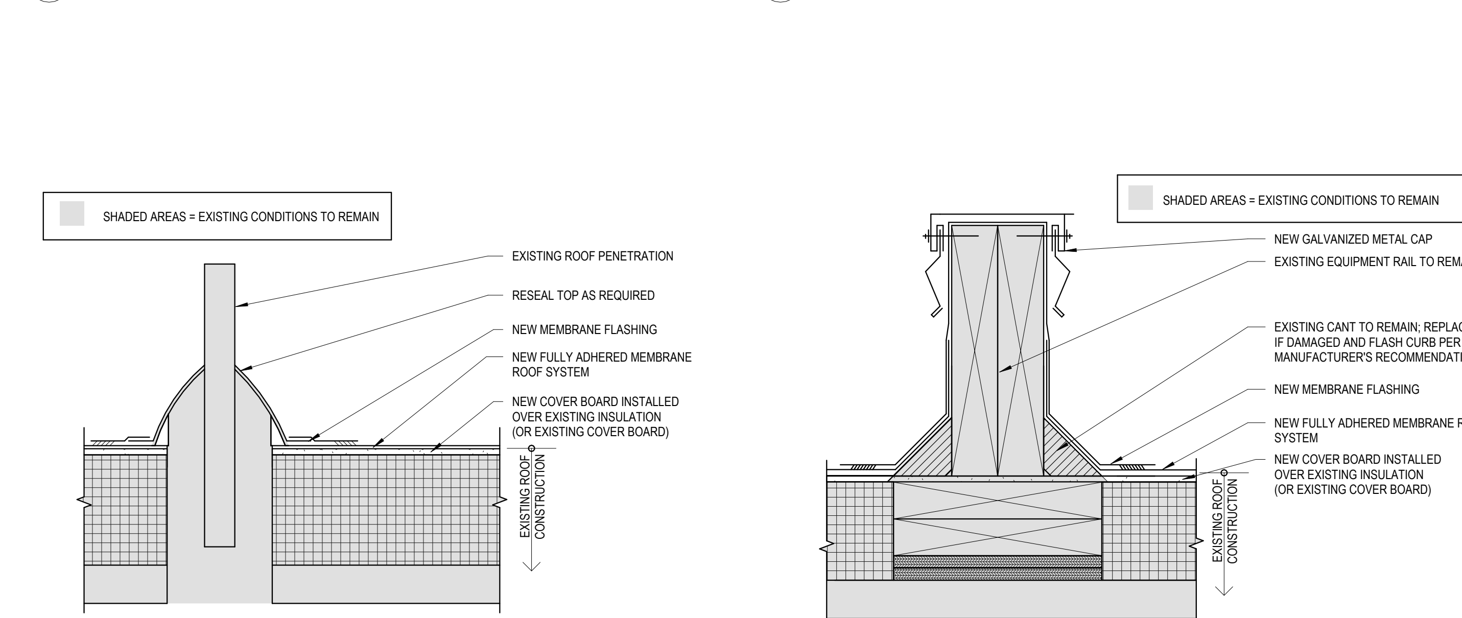
5 Typical Roof Penetration Detail Scale: 3/4" = 1'-0"
